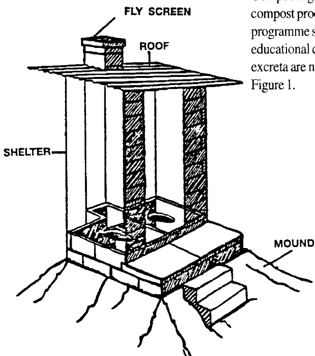
Figure 1. Composting latrine
