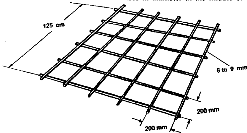
Figure 10. Reinforcement grid
