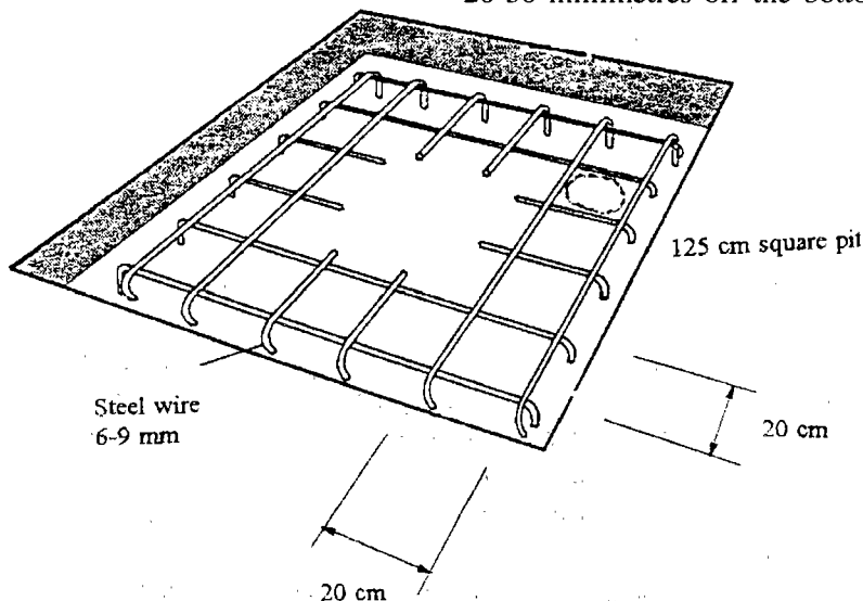
Figure 11. Laying the grid in the pit
